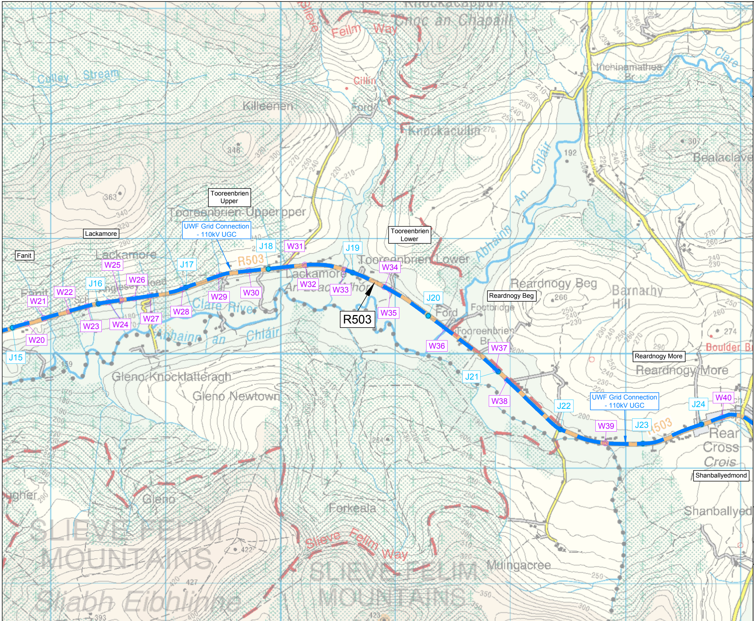
AA Figure 2 Layout of the 110kV UGC outside of the Mountphilips Substation Site
